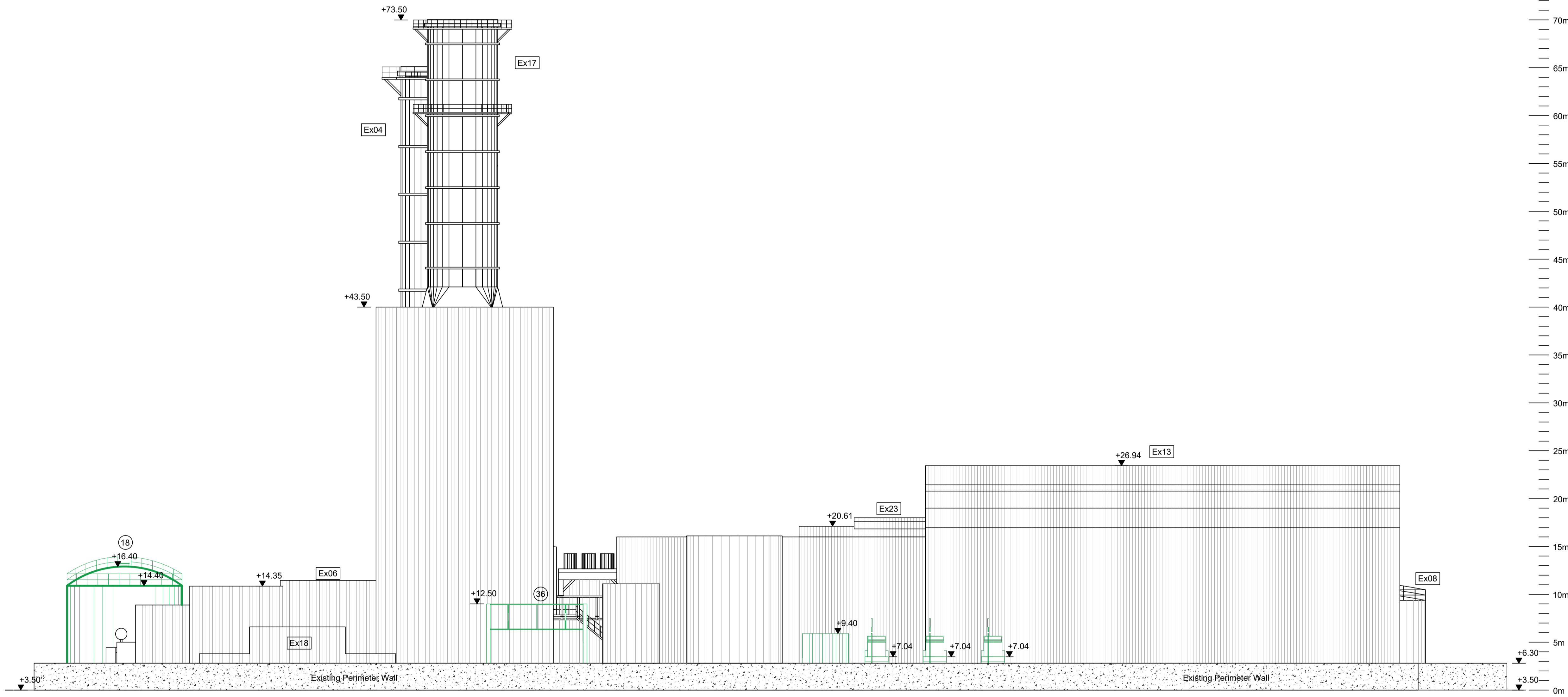
West Elevation 1:250
